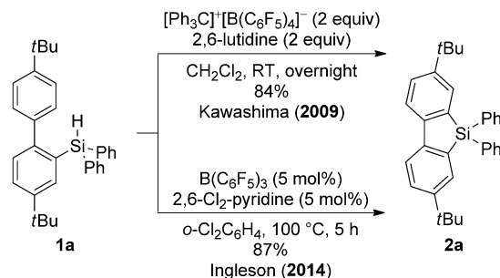
Scheme 1. Syntheses of dibenzosiloles by Friedel–Crafts-type reactions.
