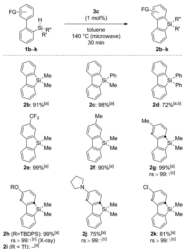
Scheme 3. Substrate scope of the Friedel–Crafts-type C–H bond silylation for the synthesis of monofunctionalized dibenzosiloles with different substituents at the silicon atom. rs = regioselectivity; TBDS = tert -butyldiphenylsilyl; Tf = trifluoromethanesulfonyl. [a] Reactions were performed on a 0.2 mmol scale. Yields of isolated products after purification by flash chromatography on silica gel. [b] With 3a (5 mol%) and 60 min reaction time. [c] The other regioisomer was not detected by GLC or NMR analysis. [d] Low conversion. With 3c (5 mol%) and 60 min reaction time, a complex mixture was obtained.
