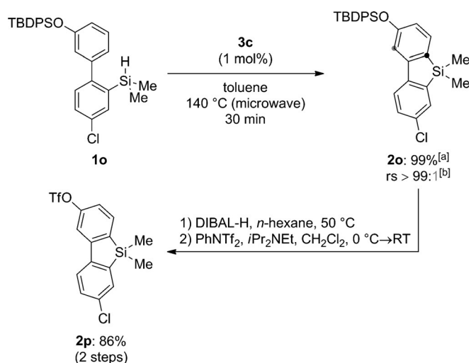
Scheme 5. Synthesis of an orthogonally difunctionalized silole monomer. DIBAL-H = diisobutylaluminum hydride. [a] Reaction was performed on a 0.2 mmol scale. Yield of isolated products after purification by flash chromatography on silica gel. [b] The other regioisomer was not detected by GLC or NMR analysis.
