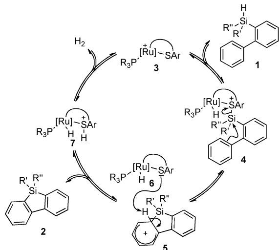
Scheme 2. S Ar -based C–H silylation (top left; FG = functional group), catalyst 3 with BAr F 4 − = tetrakis[3,5-bis(trifluoromethyl)phenyl]borate (top right), and proposed catalytic cycle with simplified catalyst structure (bottom; BAr F 4 − counterion omitted for clarity).
