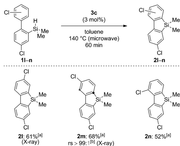
Scheme 4. Substrate scope of the Friedel–Crafts-type C–H bond silylation for the synthesis of difunctionalized silole monomers. [a] Reactions were performed on a 0.2 mmol scale. Yields of isolated products after purification by flash chromatography on silica gel. [b] The other regioisomer was not detected by GLC or NMR analysis.
